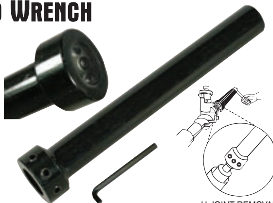
U-JOINT REMOVAL
