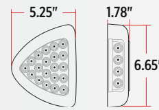
AMBER TURN & MARKER TO GREEN AUX. TLED-PSHXG
