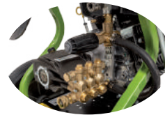
External by-pass system to a tank on JET3500-BP & JET4000-BP
