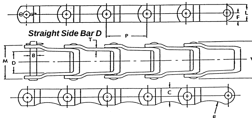
"DIMENSIONS - INCHES"
