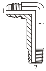
MJ X MP 90° X-LONG
